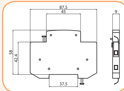
NC + NC
